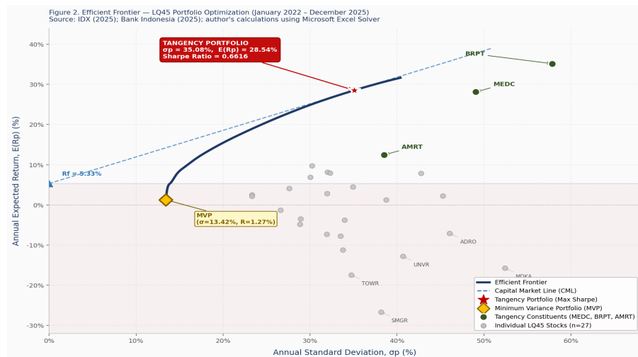
Figure 1. Efficient Frontier — LQ45 Portfolio Optimization (January 2022 to December 2025)
